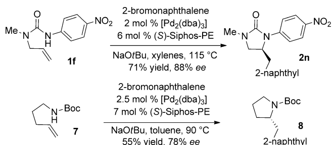
Scheme 1. Stereochemistry of urea versus pyrrolidine formation.
